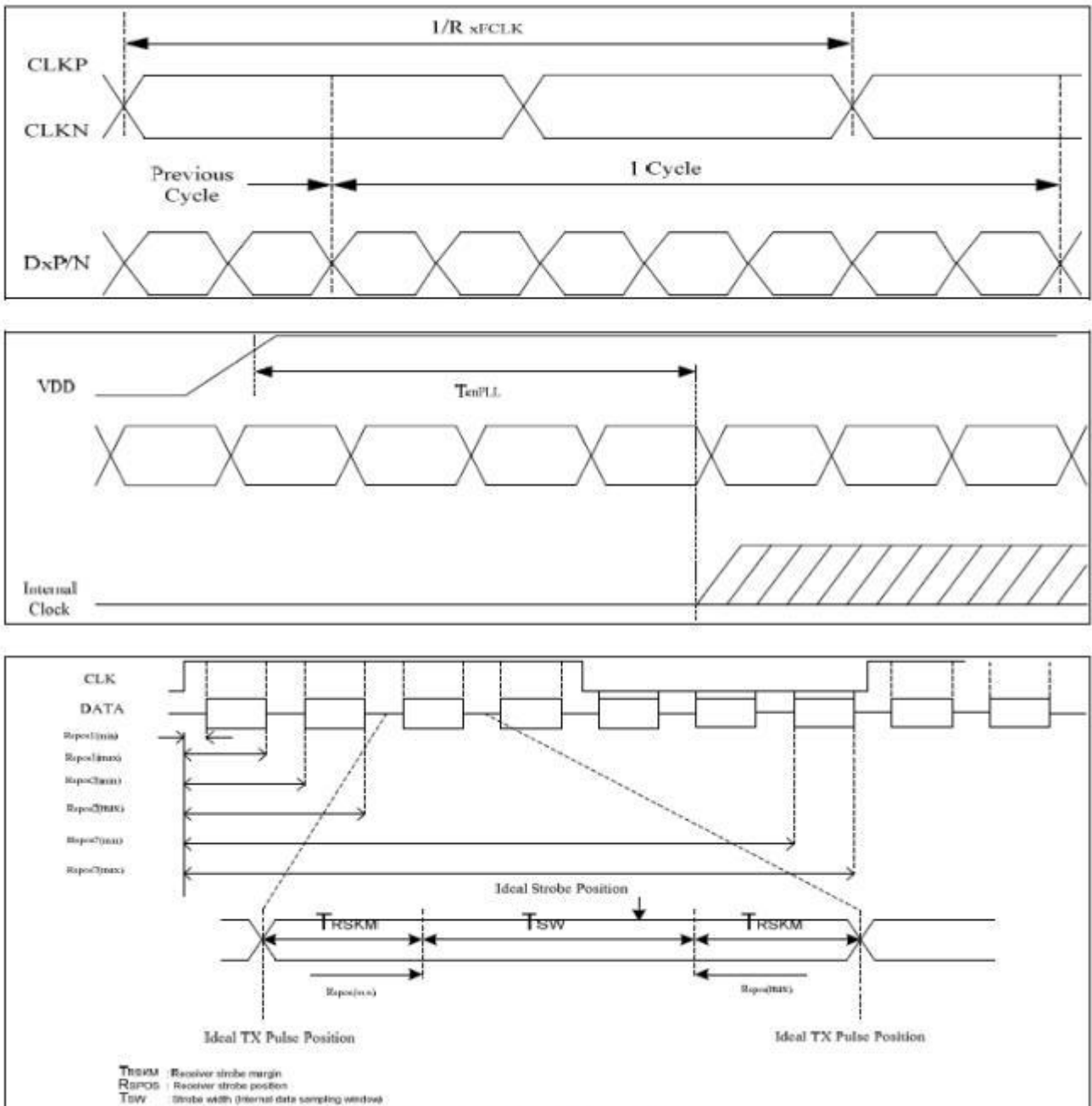
Figure 13.3: LVDS figure
