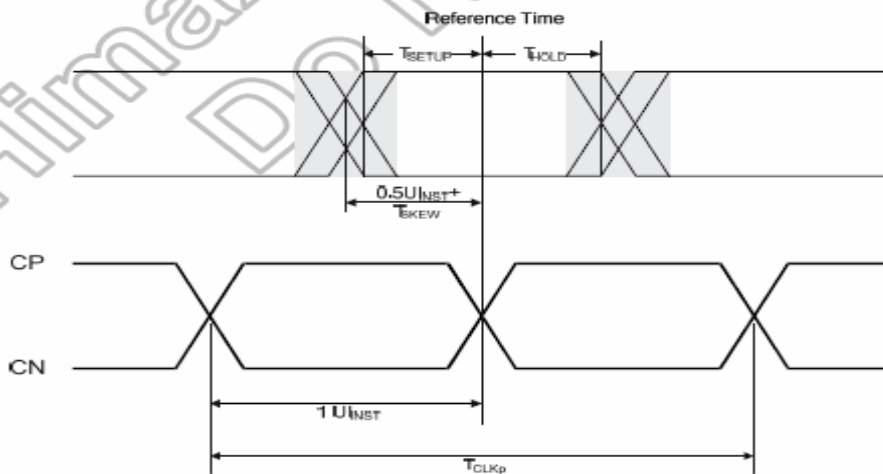
Figure 7.10: Data to Clock Timing Definitions
