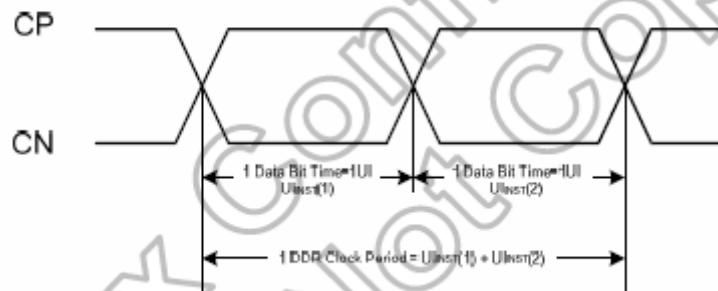
Figure 7.9: DDR Clock Definition
