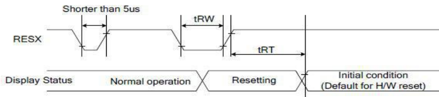
Figure 126: Reset Timing
