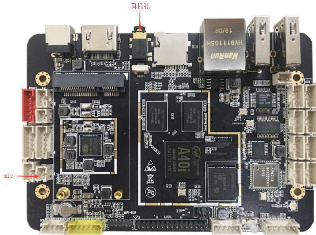
Earphone port
